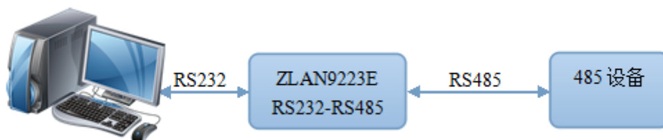
Figure 1 Connection Diagram
